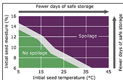
Figure 1. Safe storage charts for flax
